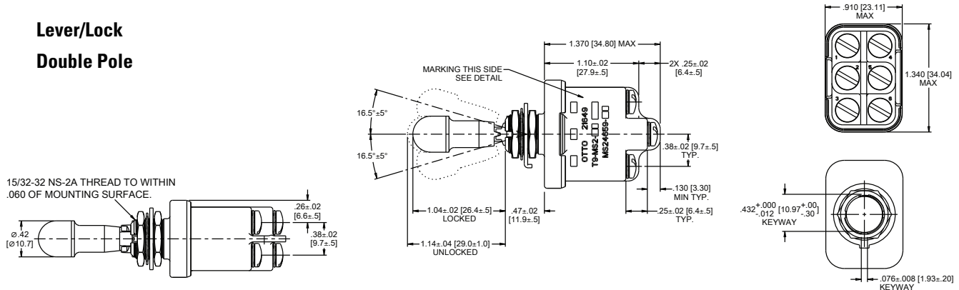
LOCKING CONFIGURATIONS
