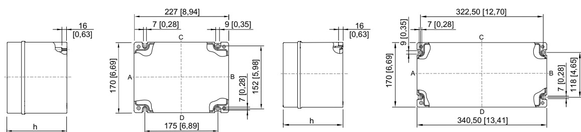
8146/.05. 8146/.051: h = 91 mm [3.58 inch] 8146/.052: h = 131 mm [5.16 inch]
