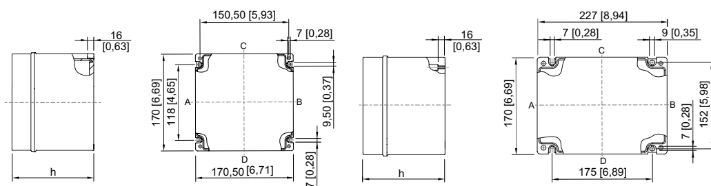
8146/.05. 8146/.051: h = 91 mm [3.58 inch] 8146/.052: h = 131 mm [5.16 inch]
