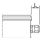
8118/1.1. Enclosure SZ 1
