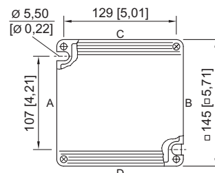
8118/1.3. Enclosure SZ 3
