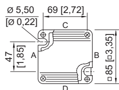
8118/1.1. Enclosure SZ 1
