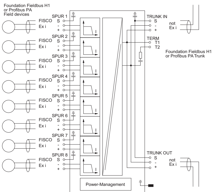
Connection diagram 9411/2.
