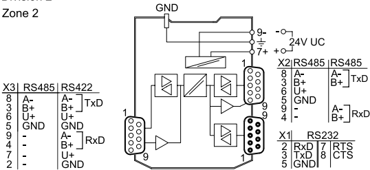
Connection diagram 9185/12
