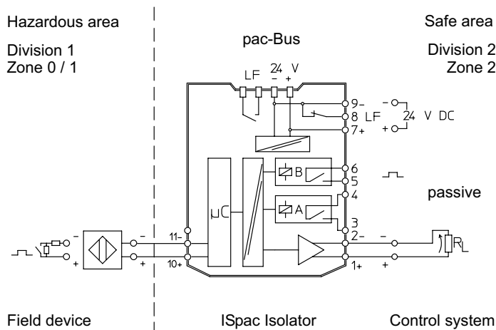
Connection diagram 9146/10-11-12
