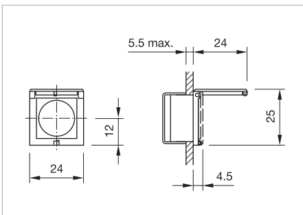
Dimensions [mm] for Part No. 61-9921.0
