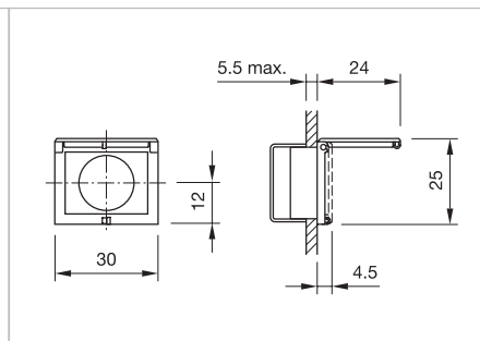
Dimensions [mm] for Part No. 61-9922.0
