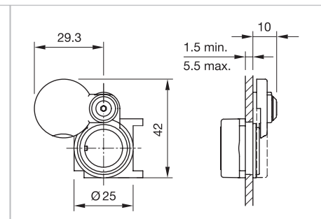
Dimensions [mm] for Part No. 61-9924.0
