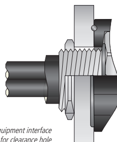
Protruding equipment interface seal for threaded entries
