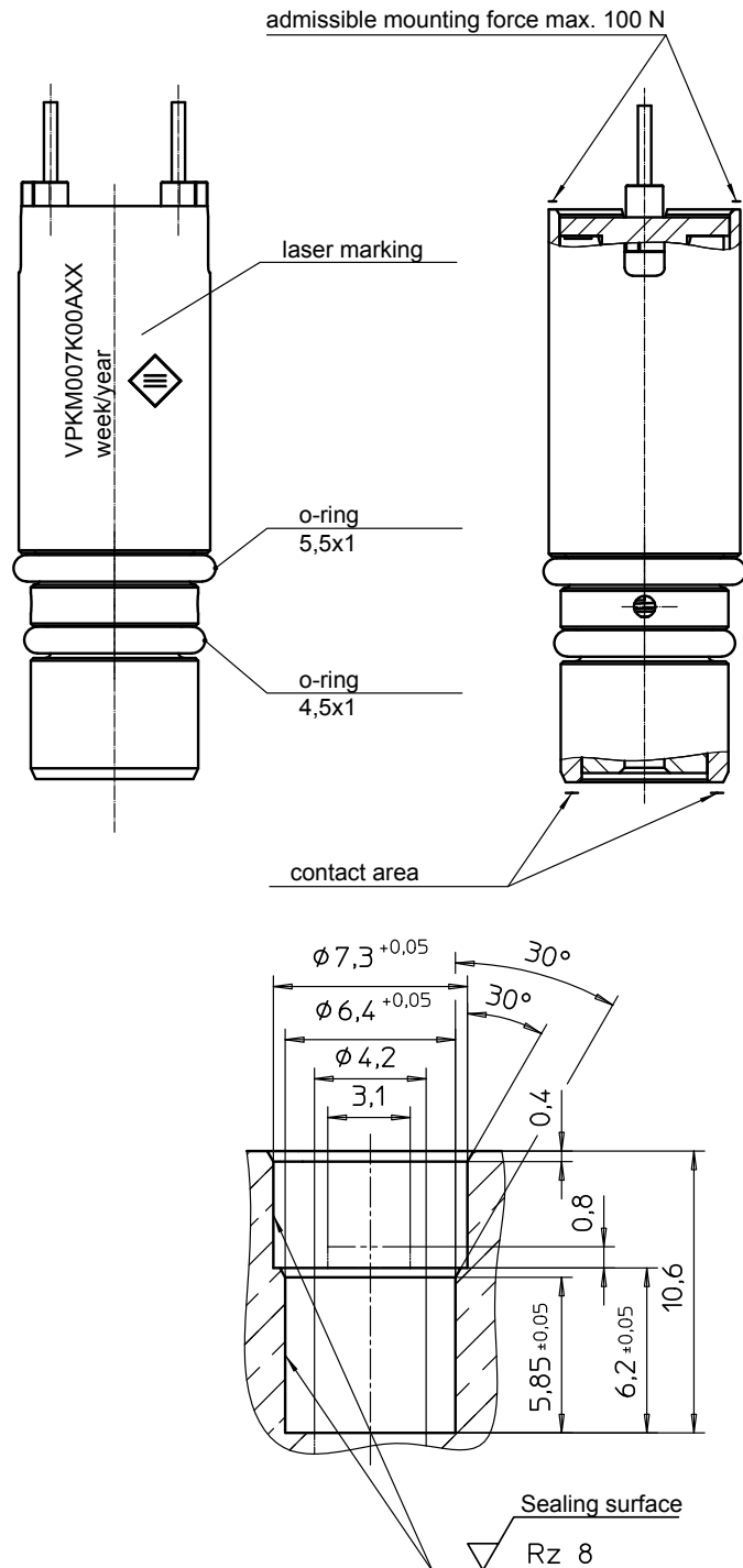
Fig. 5: Connection diagram for V PK M 007 K00 A03/A04
