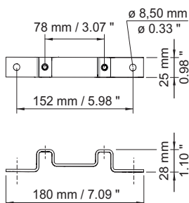
Backstrap bracket
