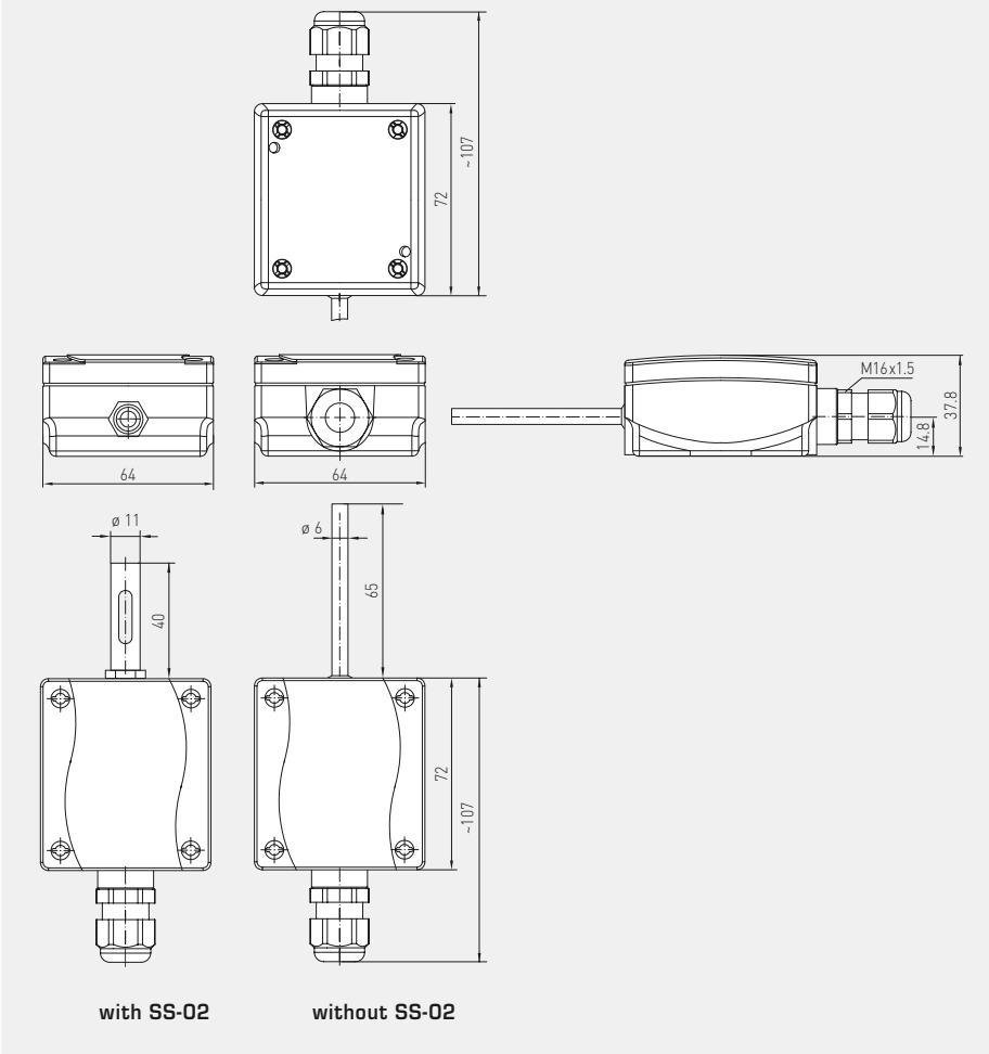
Dimensional drawing
