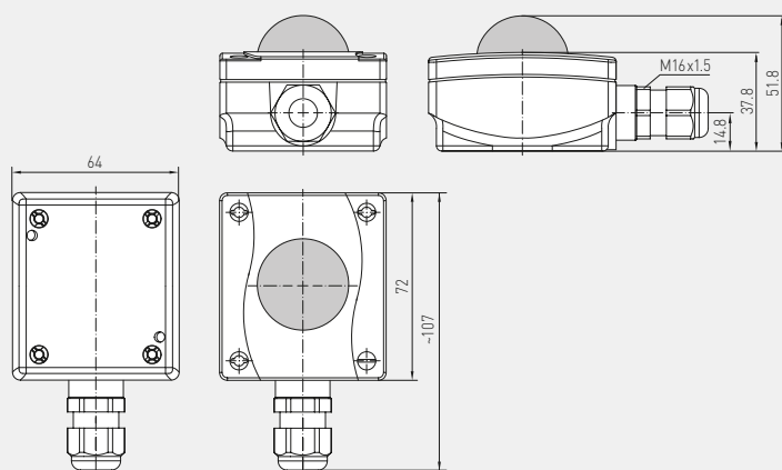
Dimensional drawing
