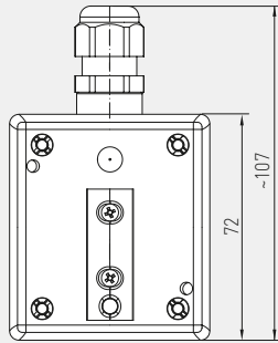
Dimensional drawing
